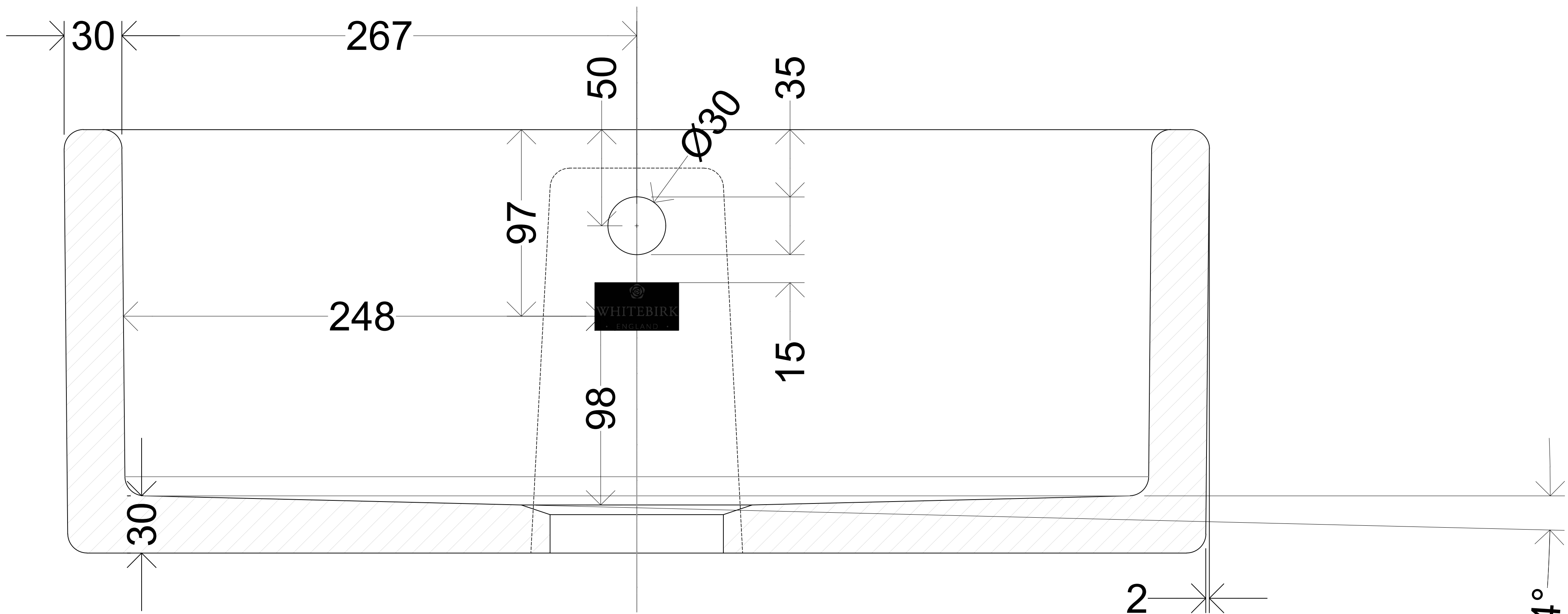
SECTION
