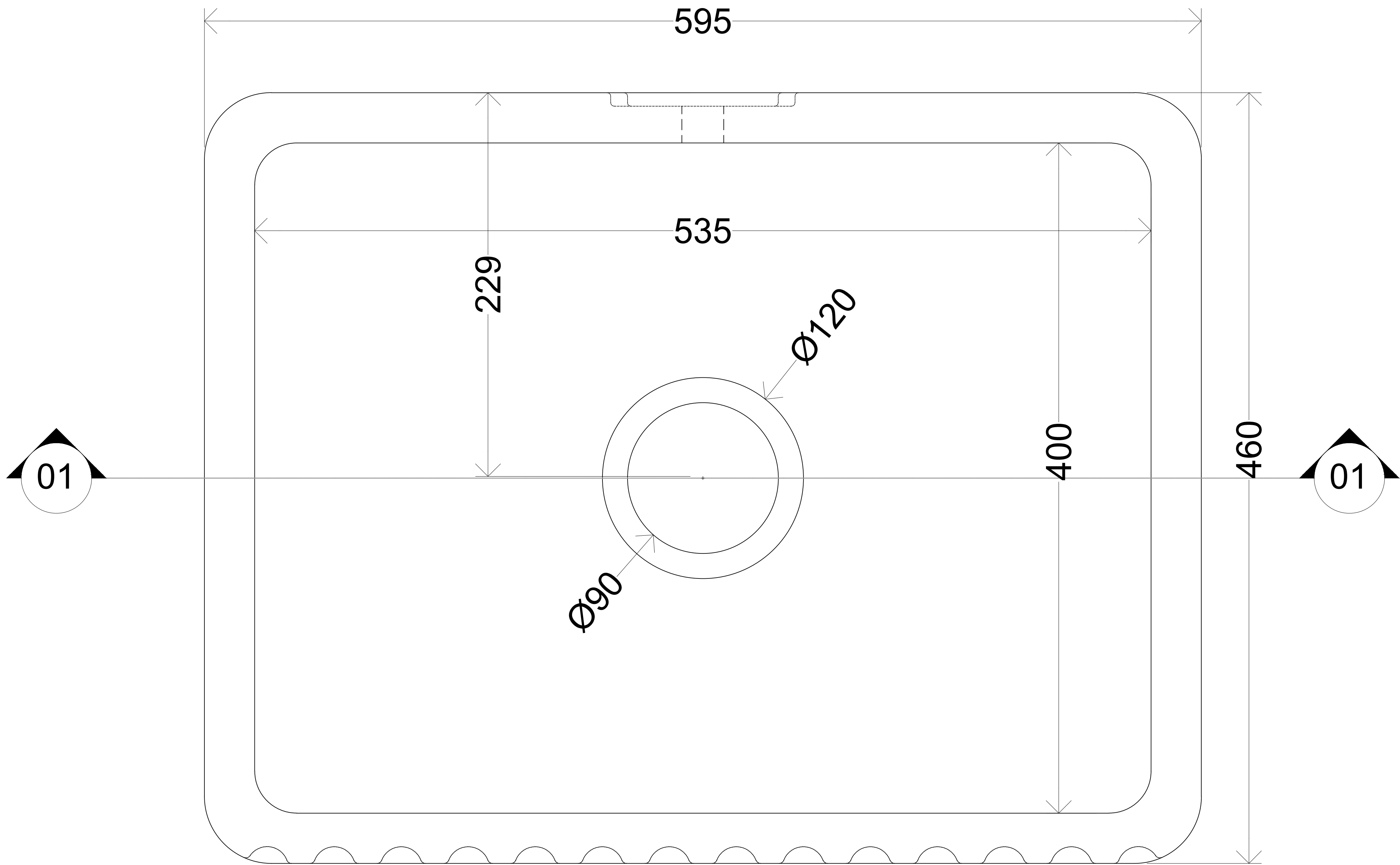
PLAN
