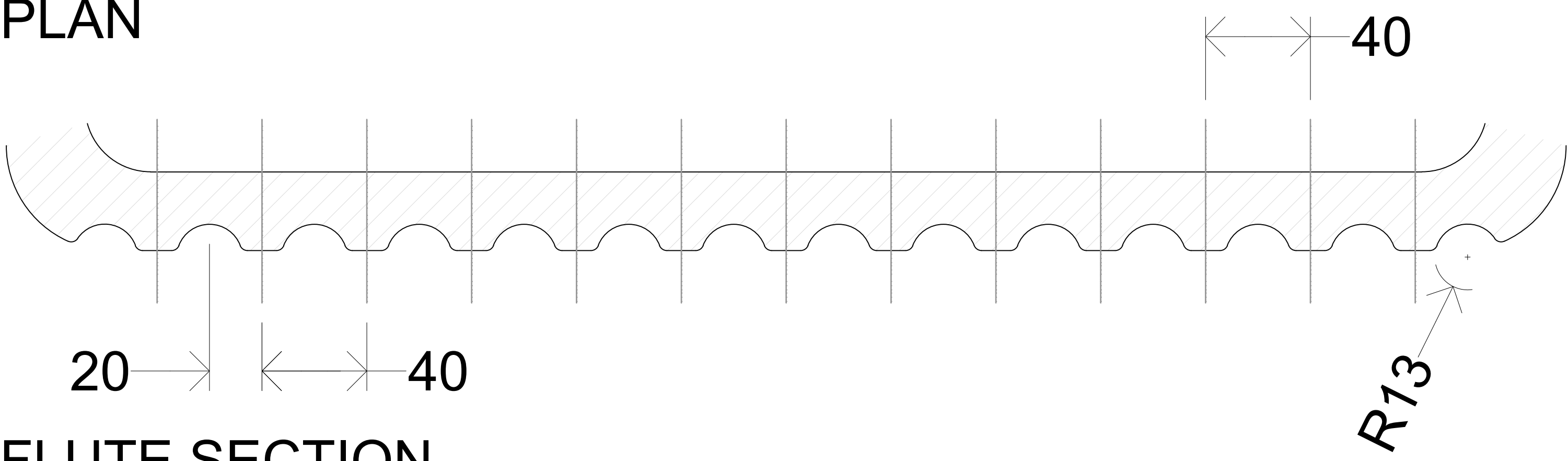
FLUTE SECTION
